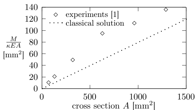
Figure 1: Normalized bending stiffness of a foam in dependence of specimen cross section
